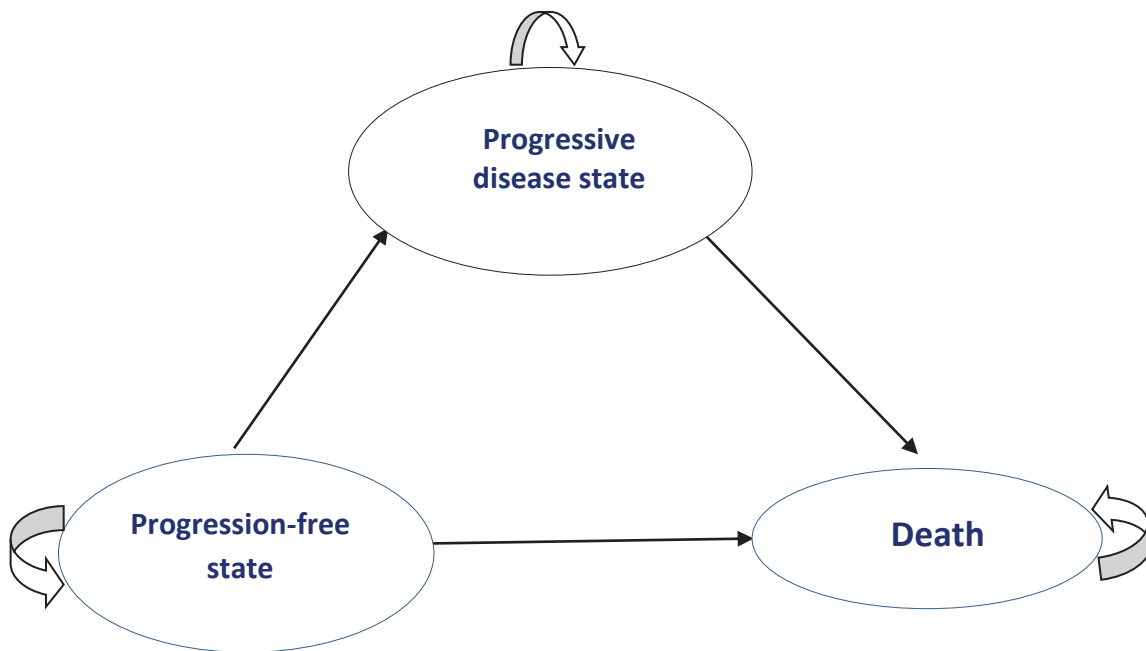
Figure 14: Markov Model
